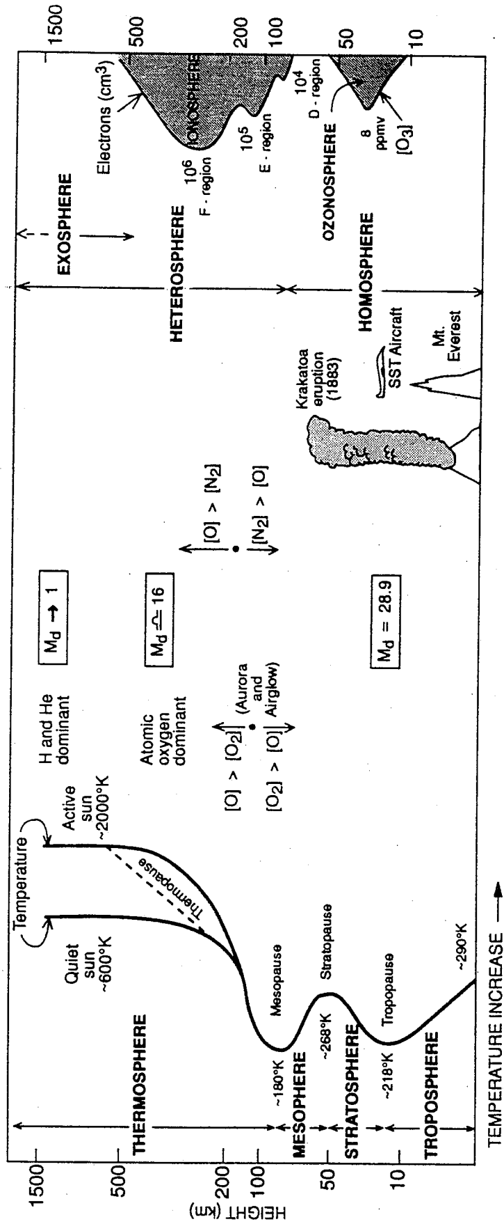
Figure 3.1. Two ways of dividing the atmosphere: by temperature structure (left side) and by composition (right side). The change in the apparent molecular weight of air ( M_d ) due to the changing composition of the atmosphere with height is shown in the center.
